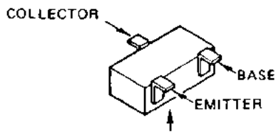
Marked Surface 2SC1623(L6) (Q7701, Q7704, Q7801, Q7804)
