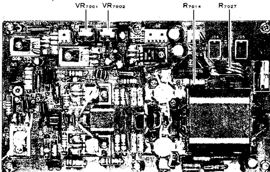
PA (RF Power Amp) Unit Test & Alignment Points
