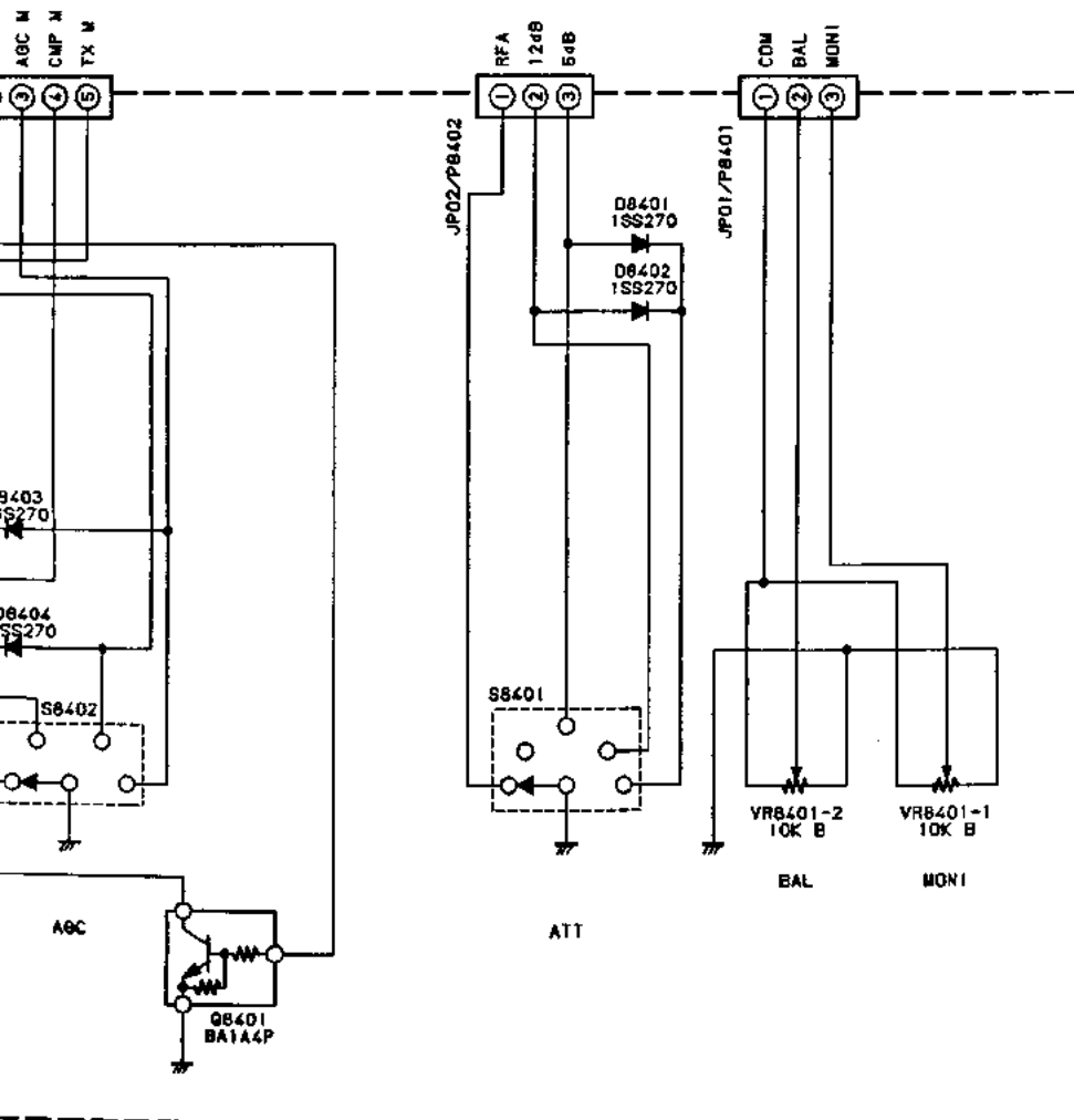
(SW B UNIT schematic diagram)
