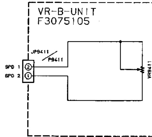
(VR B UNIT schematic diagram)
