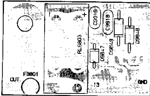
(obverse view of "component" side)
