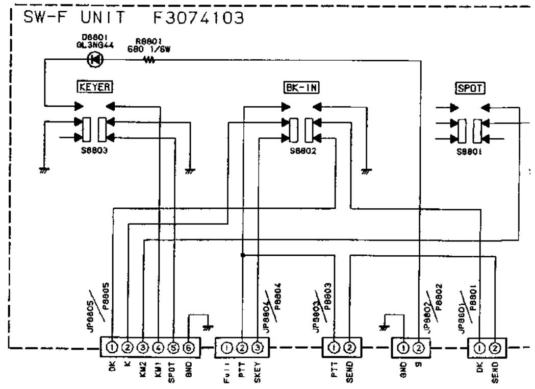
(SW F UNIT schematic diagram)
