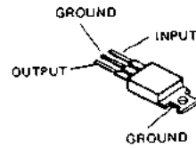
μPC7805H (Q4013)
