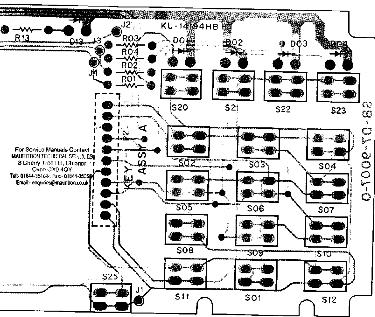
(obverse view of "component" side)
