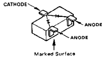
1SS184 (B3) (D4017, D4018, D4019, D4020, D4021)
