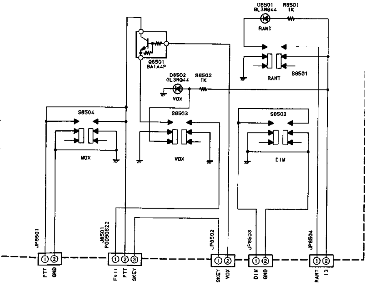
(SW C UNIT schematic diagram)
