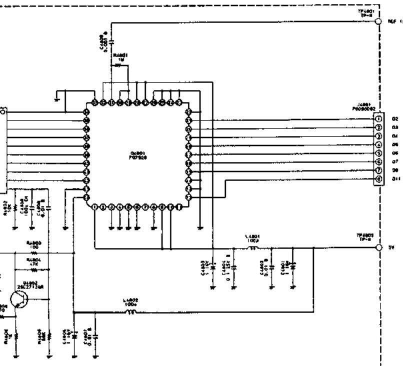
(SHIFT DDS UNIT schematic diagram)
