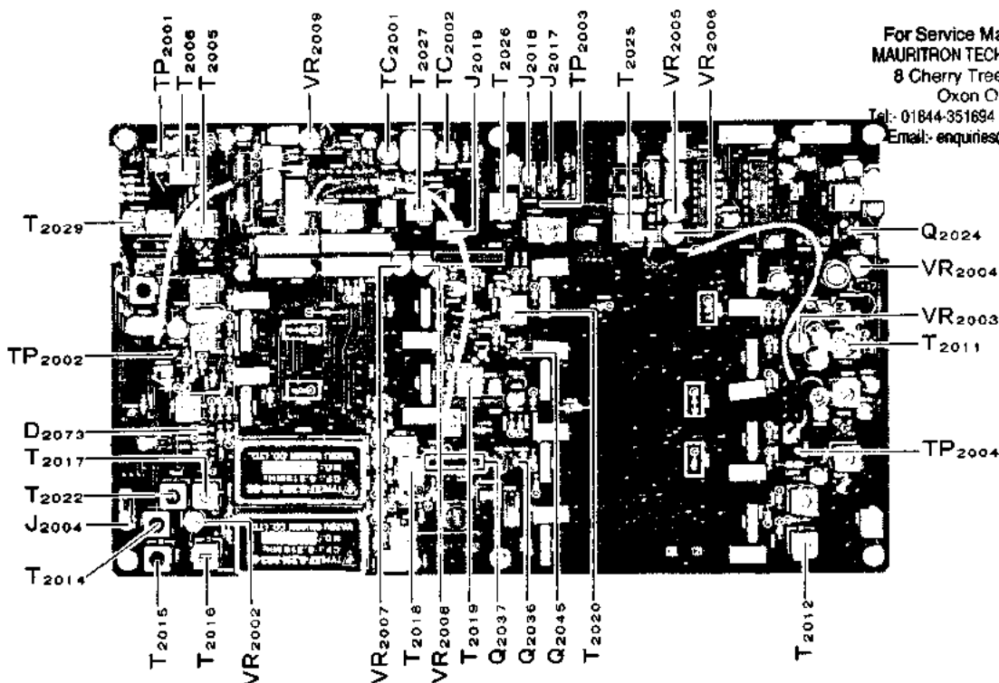
IF Unit: Receiver Test & Alignment Points
