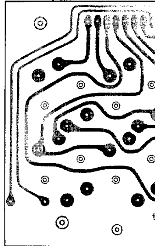
(obverse view
