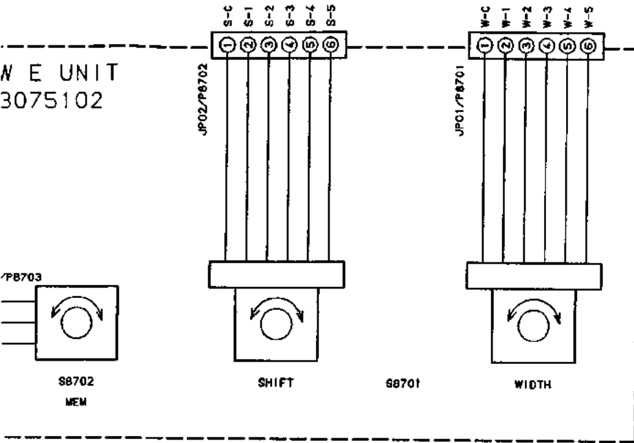
(SW E UNIT schematic diagram)
