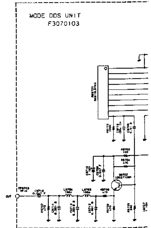
(MODE DDS UNIT schematic diagram)
