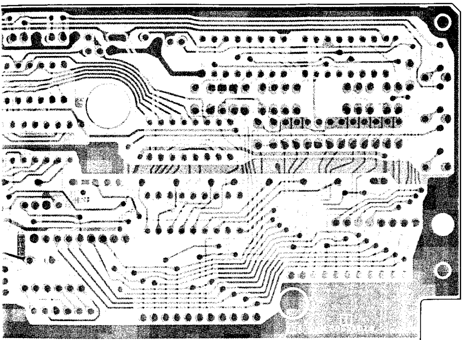
(obverse view of "solder" side)
