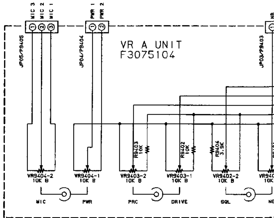
(VR A UNIT schematic diagram)
