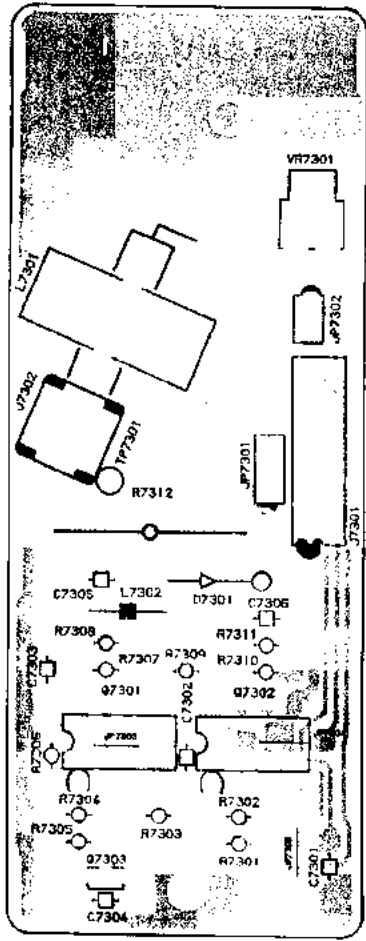
(obverse view of "component" side)
