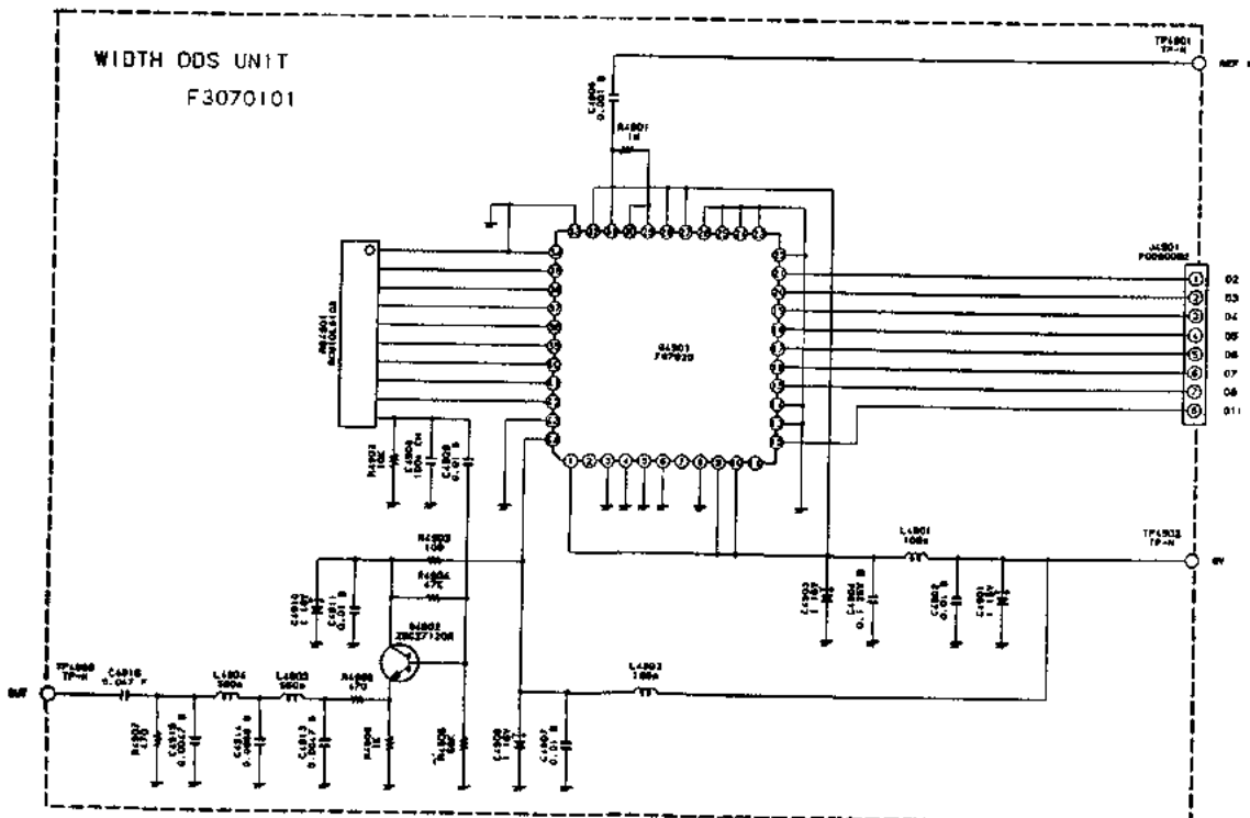
(WIDTH DDS UNIT schematic diagram)
