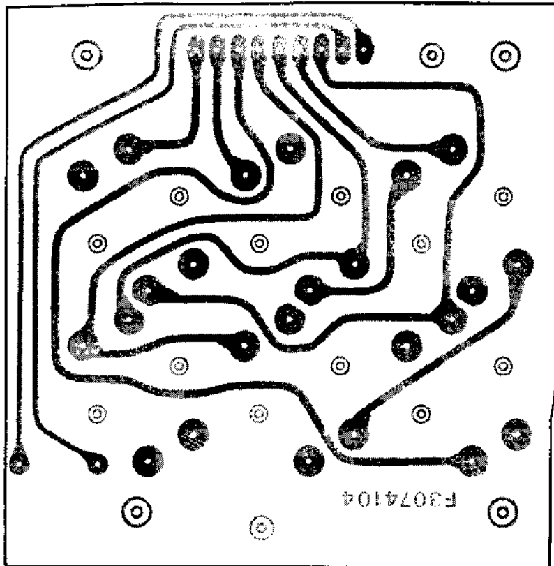
(obverse view of "solder" side)
