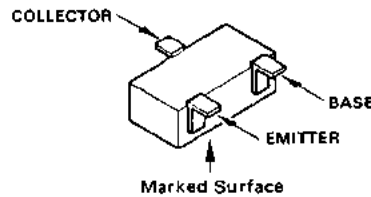
FA1A4M (L33) (Q4051, Q4053, Q4055, Q4057, Q4065, Q4066, Q4067, Q4069, Q4070)
