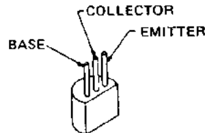
2SA733AQ (Q7605, Q7606, Q7608, Q7609)
