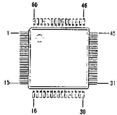
TC23SC030AF (Q7702, Q7802)
