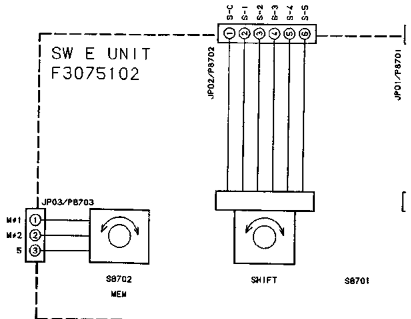
(SW E UNIT schematic diagram)
