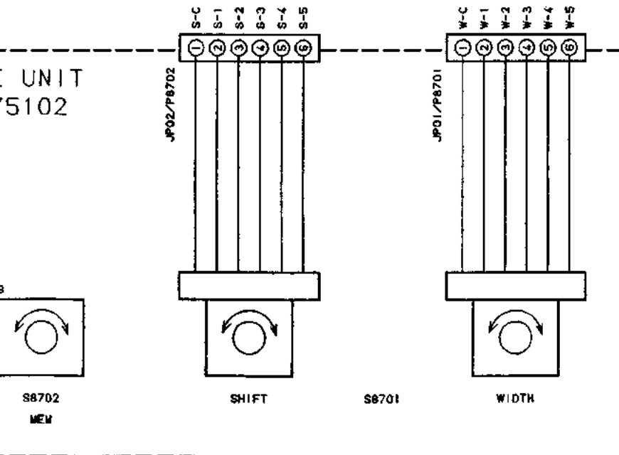
(SW E UNIT schematic diagram)
