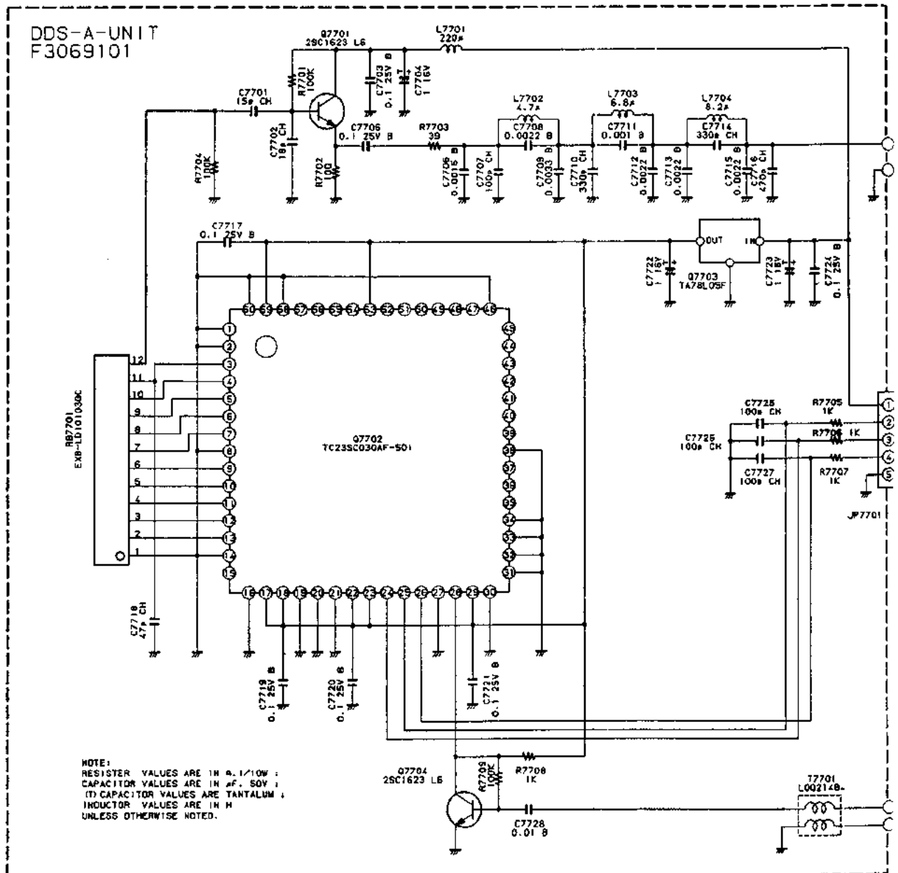
(DDS-A UNIT schematic diagram)
