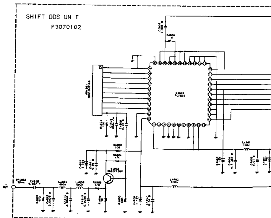
(SHIFT DDS UNIT schematic)
