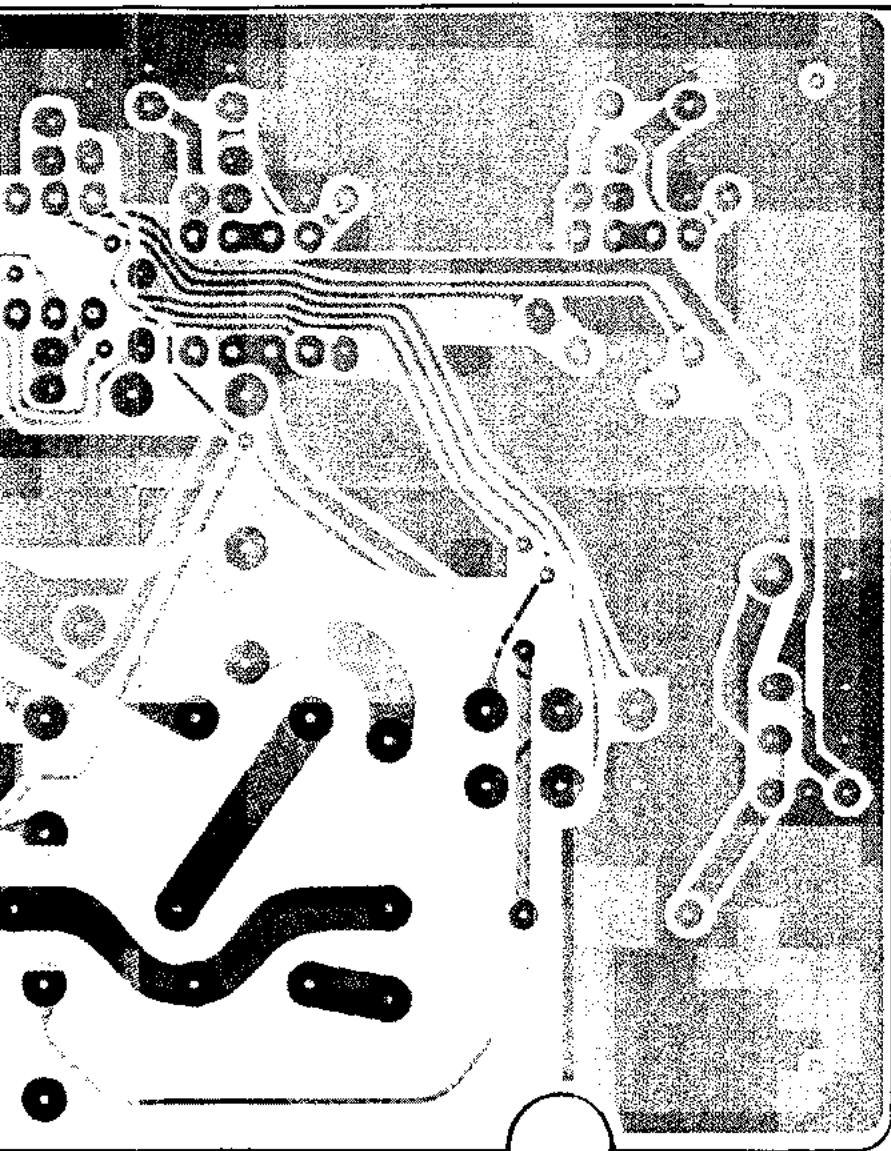
(obverse view of "solder" side)
