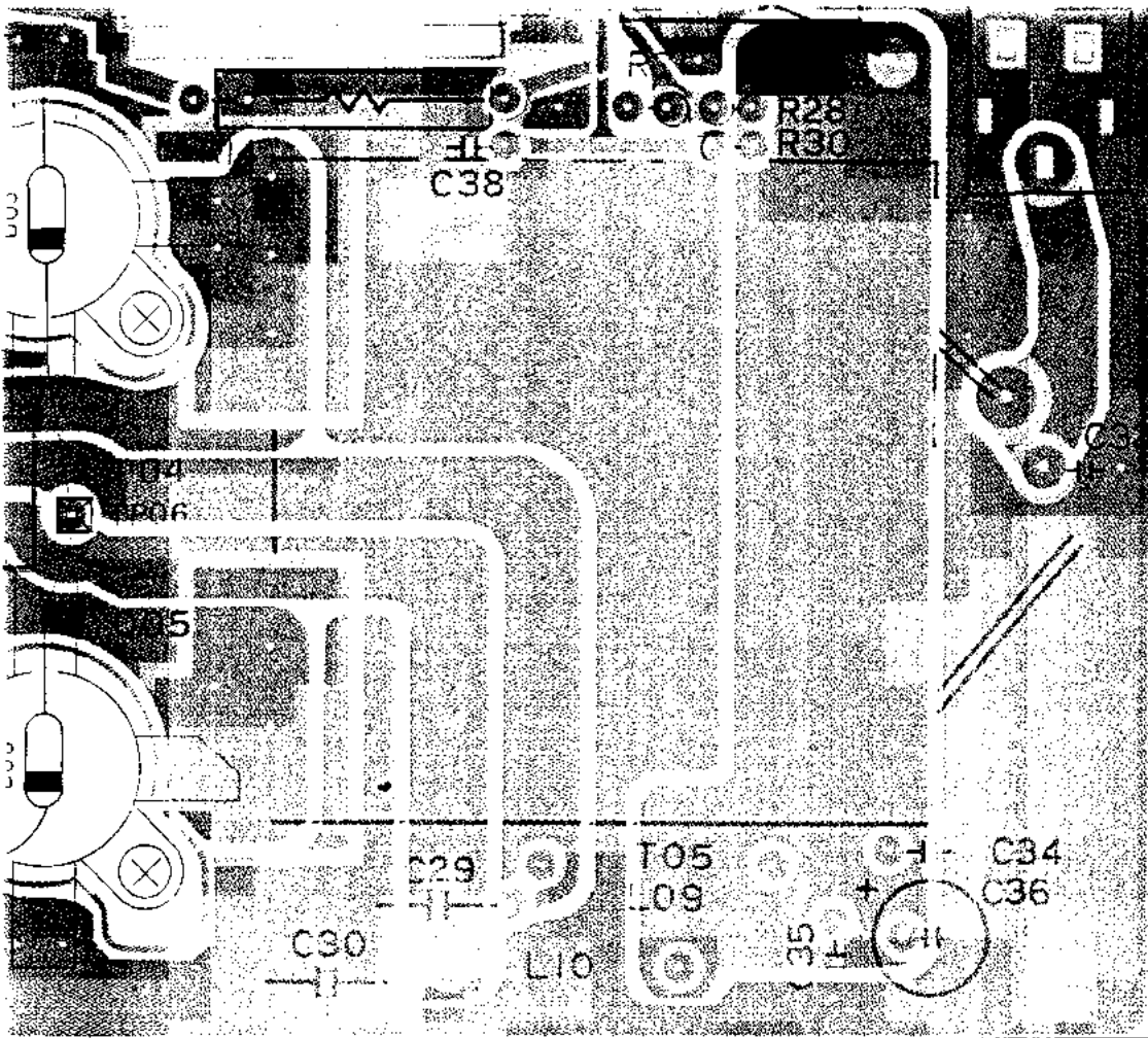
(obverse view of "component" side)
