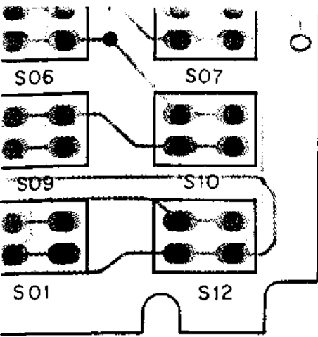
view of "component" side)
