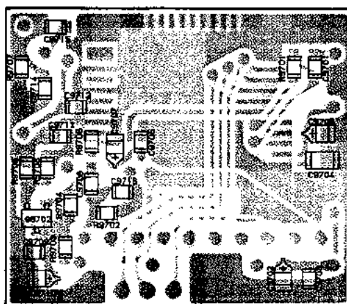
(obverse view of "chip-only" side)
