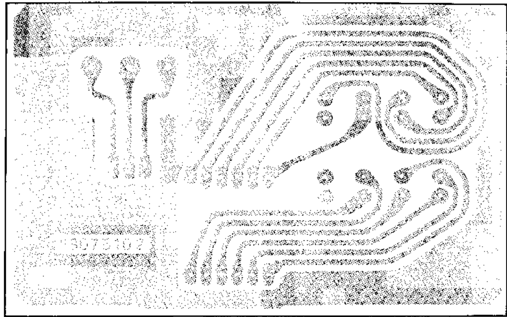
(obverse view of “solder” side)
