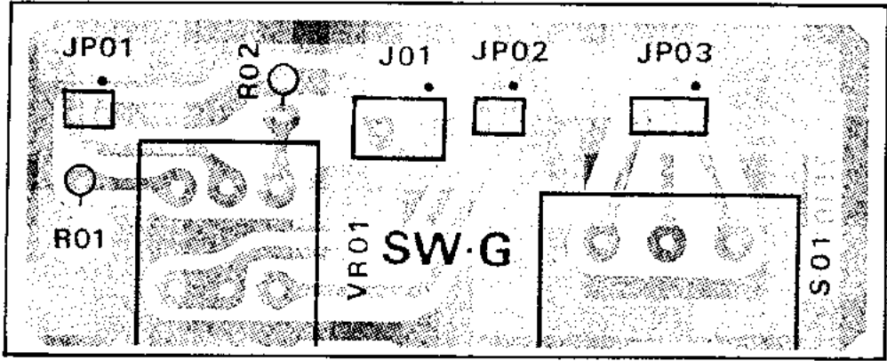
(obverse view of "component" side)
