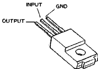
M5F79M09 (Q7620)
