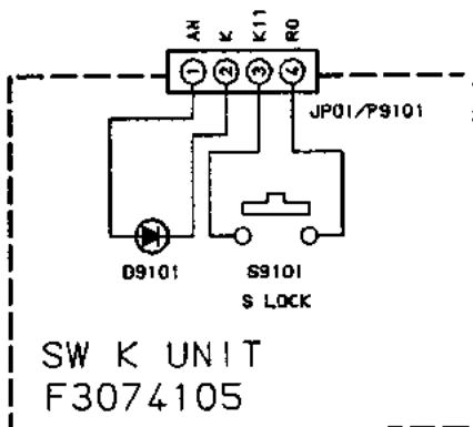
(SW K UNIT schematic diagram)
