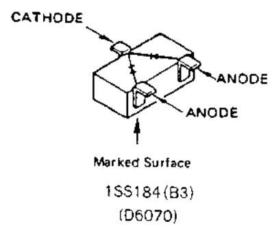
(obverse view of "chip-only" side)
