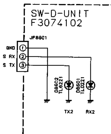
(SW D UNIT schematic diagram)
