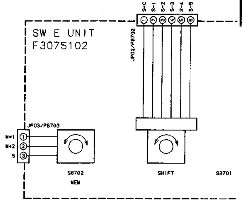
(SW E UNIT schematic diagram)
