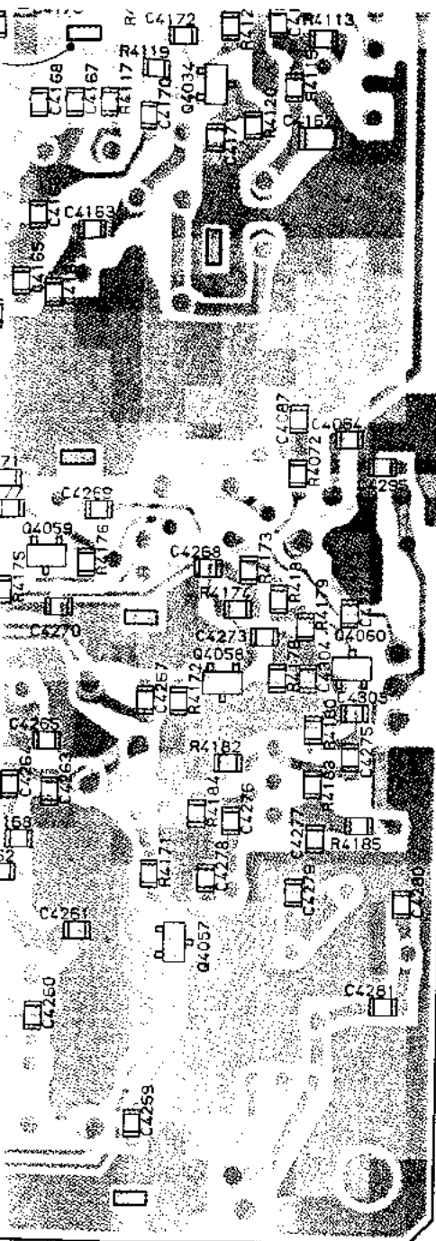
view of "chip-only" side)
