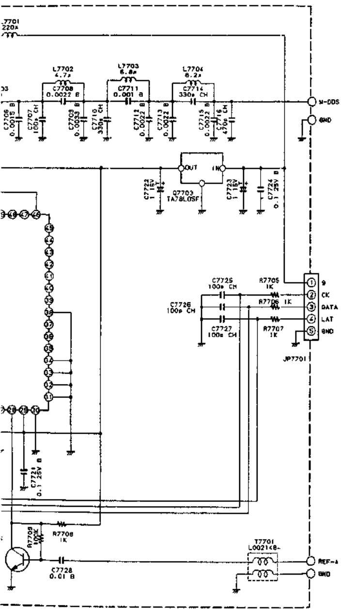
(DDS-A UNIT schematic diagram)
