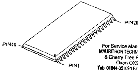
M5M82055AFP (Q5004, Q5005, Q5006, Q5007)
