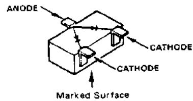
1SS181 (A3) (D4022)
