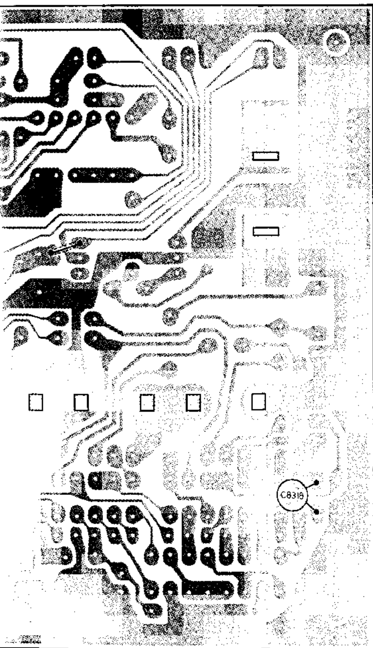
(obverse view of "chip-only" side)
