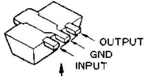
Marked Surface TA78L05F (05) (Q5048)
