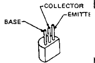
2SA684R (Q7201)
