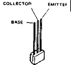
BA1A4P (Q8401, Q8501)
