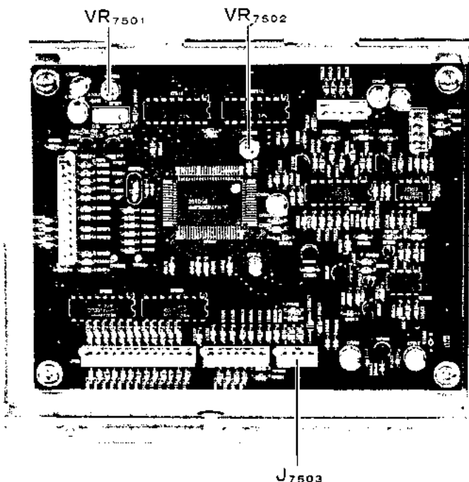
J7503 Tuner Control Unit Test & Alignment Points
