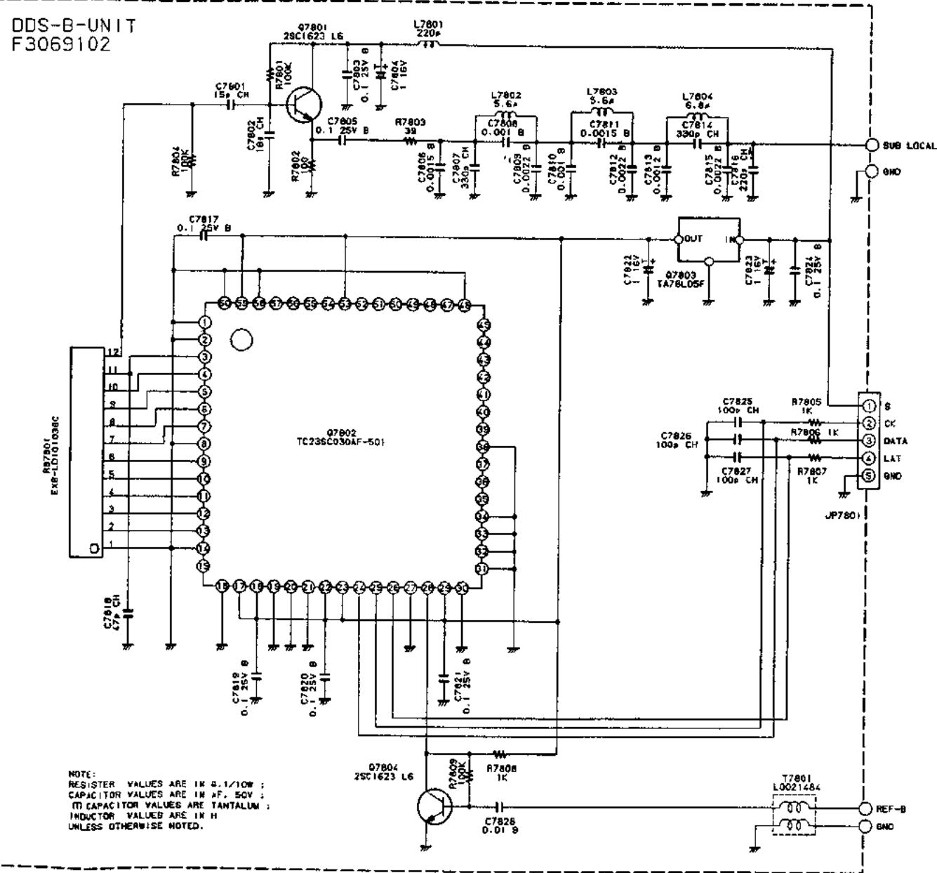
(DDS-B UNIT schematic diagram)
