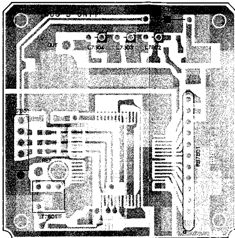
(obverse view of "component" side)
