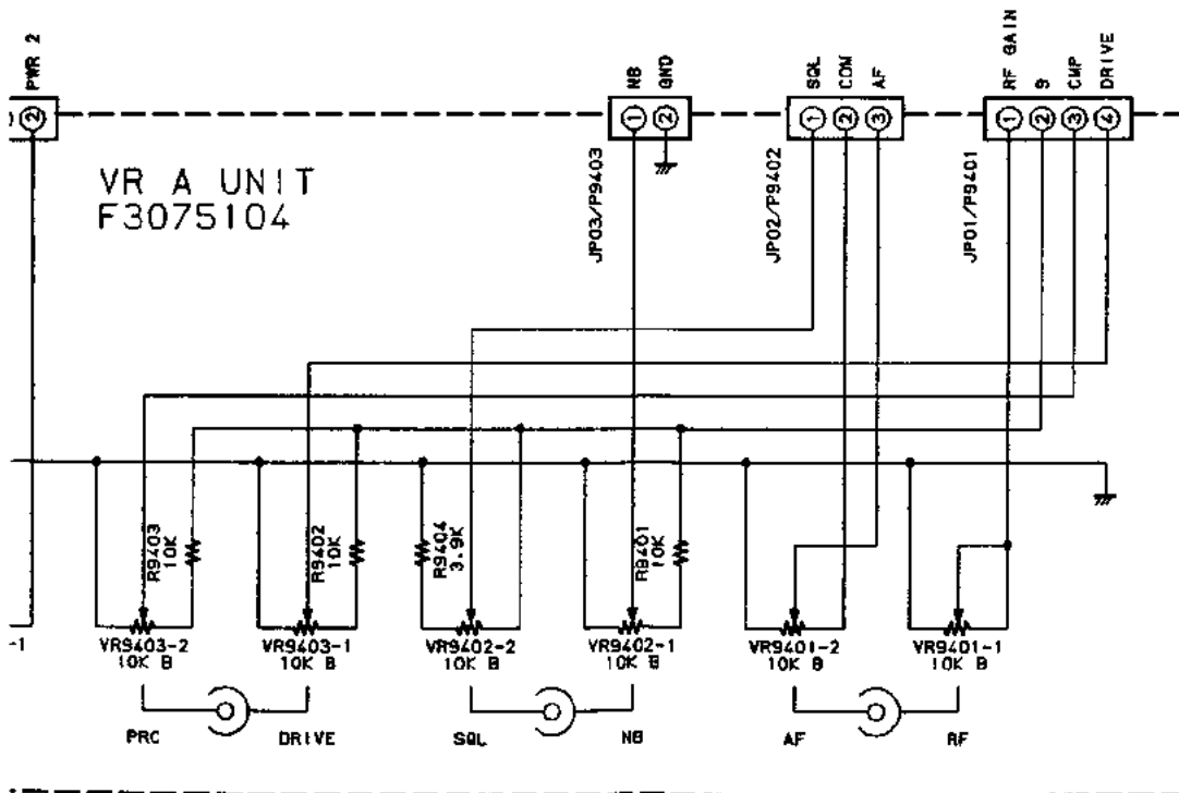
(VR A UNIT schematic diagram)
