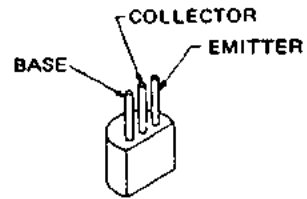
2SA733A0 (Q7605, Q7606, Q7608, Q7609)
