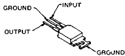
MC7808CT (Q7008)
