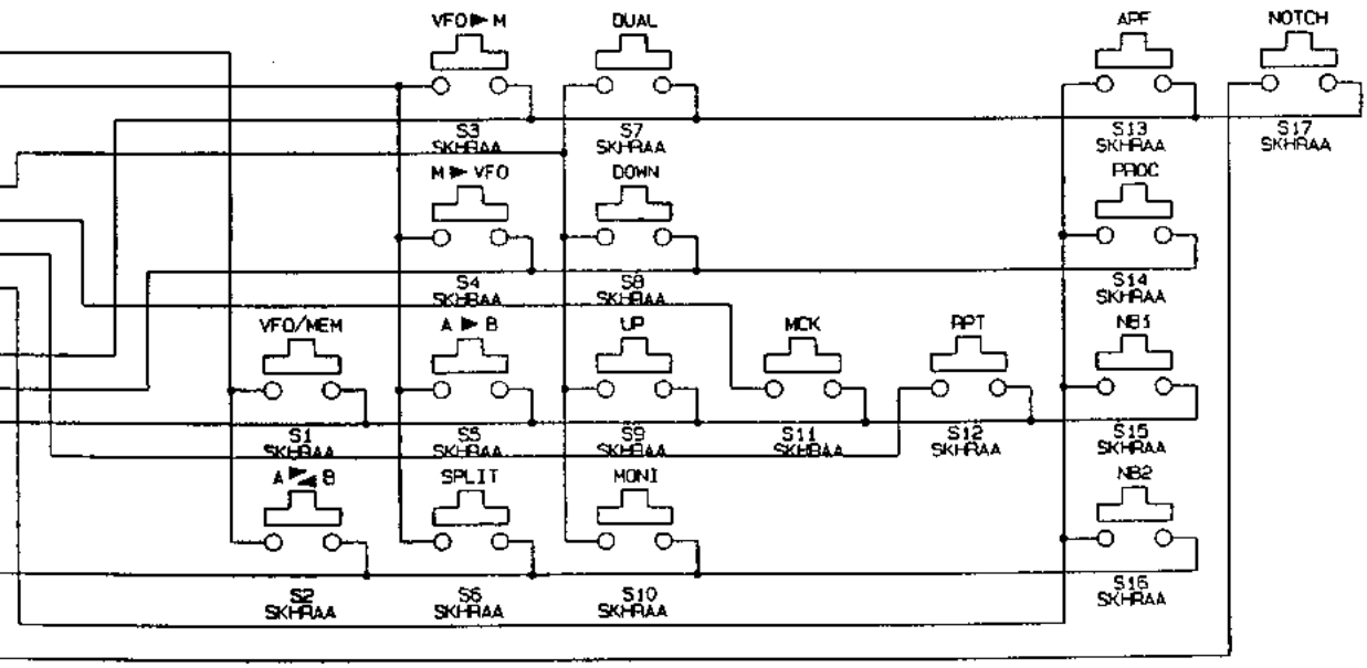
( schematic diagram )
